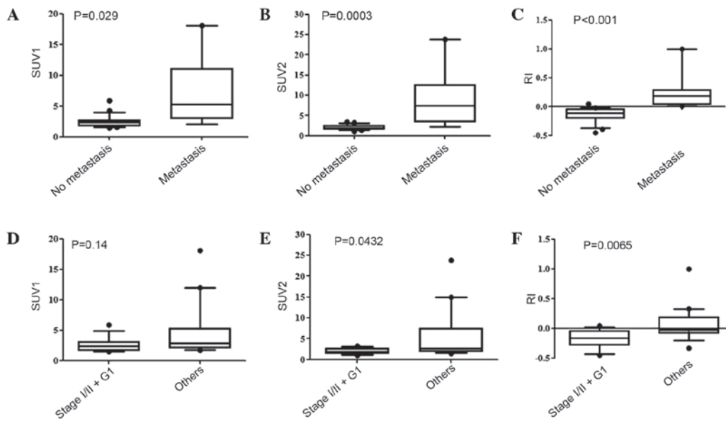
Figure 1. 18 F-fluorodeoxyglucose-positron emission tomography/computed tomography findings according to metastatic or pathological status. (A) SUV1, (B) SUV2 and (C) RI according to metastatic status in RCC patients. (D) SUV1, (E) SUV2 and (F) RI according to pathological status in RCC patients. Dots indicate raw values. SUV1/2, standardized uptake value at 1/2 h; RI, retention index; G, grade.
