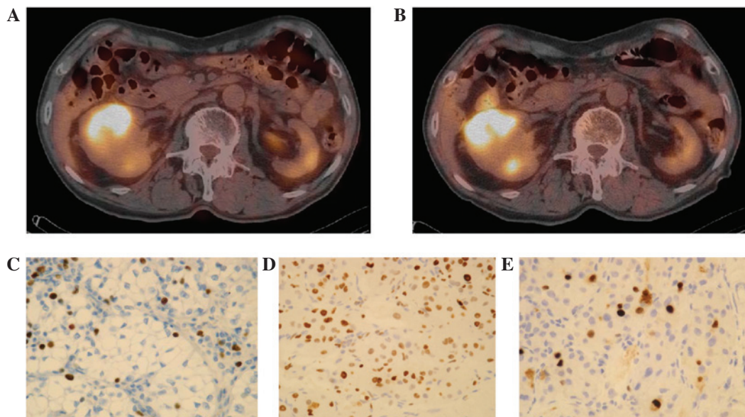
Figure 2. Representative images from a 79-year-old patients with renal cell carcinoma (pathological Tumor 3a Node 0 Metastasis 1 ). 18 F-fluorodeoxyglucose-positron emission tomography/computed tomography: (A) SUV1, 11.97 ng/ml; and (B) SUV2, 14.97 ng/ml. The RI index was 25.06%. Immunohistochemical analysis revealed potent expression of (C) Ki-67 (D) minichromosome maintenance 2 and (E) topoisomerase II \alpha . SUV1/SUV2, standardized uptake value at 1 / 2 h.
